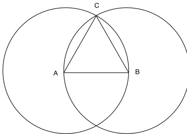
Figure 34.1 Diagram for Elements Proposition I.1
