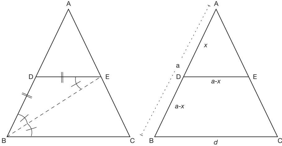
Figure 34.2 Diagrams for Lamy's example
