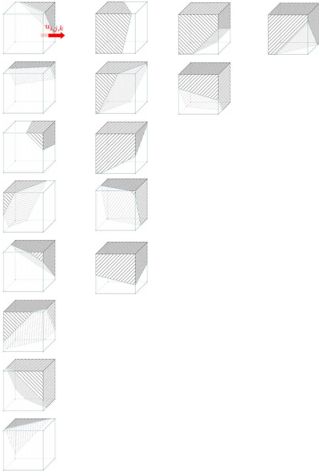
Fig. 19. Basic types of cut-cells for the skew-symmetric discretization of the convective terms for u_{ij,k} . In the first row, we have grouped the cut-cells having 6 velocity unknowns (the maximum possible in 3D), then 5 unknowns, 4 unknowns, and finally 3 unknowns (the minimum).
