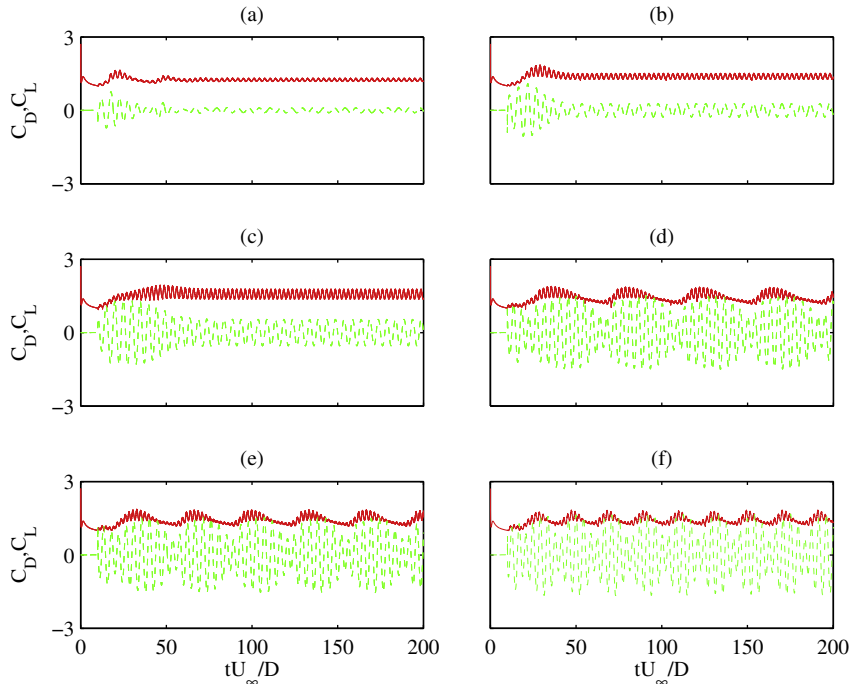
Fig. 16. Time evolution of the force coefficients (— C_D ; - - - C_L ) for the flow past an oscillating cylinder in a free-stream for S_e/S_0 equals to: (a) 0.8; (b) 0.9; (c) 1.0; (d) 1.1; (e) 1.12; (f) 1.2.
