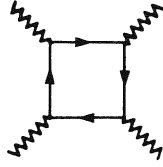
Fig. 9.9. The scattering of light by light.
