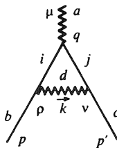
Fig. 9.20. Correction to the quark–gluon vertex.
