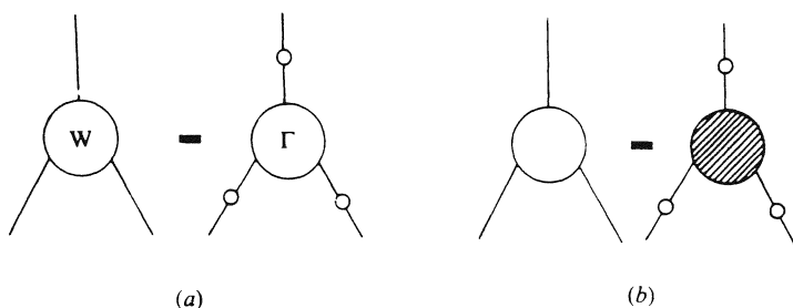
Fig. 7.1. Two representations of equation (7.88).
