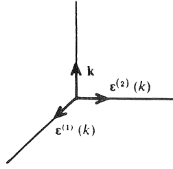
Fig. 4.1. The polarisation vectors for the electromagnetic field with momentum \mathbf{k} .
