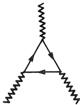
Fig. 9.8. A 3-photon vertex.
