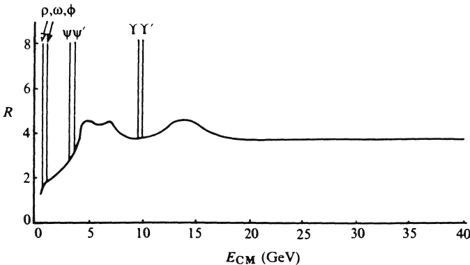
Fig. 1.13. A schematic drawing of R against centre-of-mass energy.
