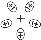
Fig. 9.10. Polarisation of a dielectric medium by a charge, or of the vacuum in QED.
