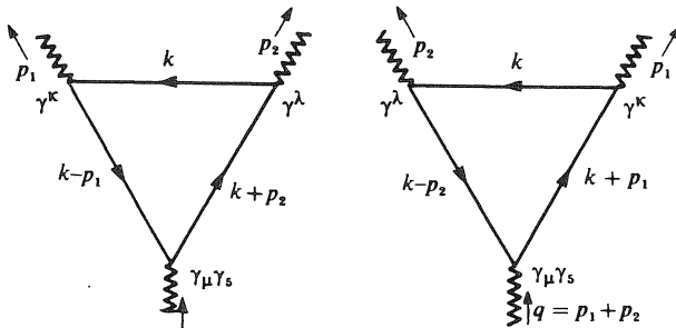
Fig. 9.24. The triangle graphs.
