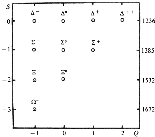
Fig. 1.3. Particles with J^P = \frac{3}{2}^+ . The right-hand axis figures are the masses in \text{MeV}/c^2 .
