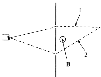
Fig. 3.7. The Bohm–Aharonov effect; a solenoid is placed between the slits.
