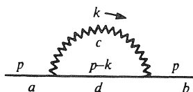
Fig. 9.16. Quark self-energy diagram.
