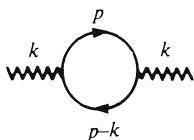
Fig. 9.6. Photon self-energy diagram.
