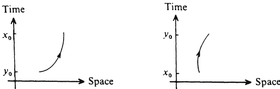
Fig. 6.3. Interpretation of equation (6.55). (See text.)
