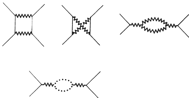
Fig. 7.10. The four diagrams in QCD contributing to q\bar{q} \rightarrow q\bar{q} to order g^4 . Wavy lines are gluon propagators, dotted lines ghost propagators.
