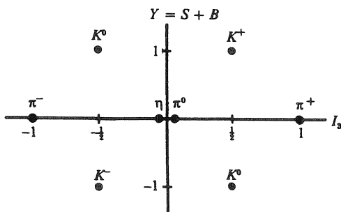
Fig. 1.5. The J^P = 0^- pseudoscalar octet of SU(3) . The masses of the (neutral) particles, in \text{MeV}/c^2 , are m(\pi) = 135 , m(K) = 498 , m(\eta) = 549 .
