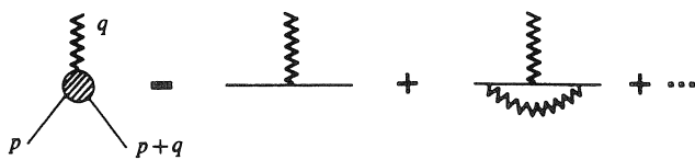
Fig. 7.5. Expansion of \Gamma_\mu(p, q, p + q) .
