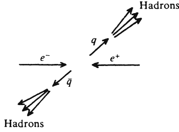
Fig. 1.12. e^+e^- annihilation into hadrons.
