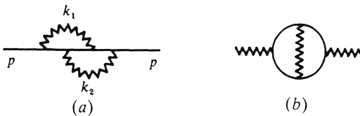
Fig. 9.13. Examples of overlapping divergences in QED.
