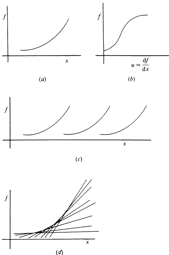
Fig. 7.3. Geometrical interpretation of the Legendre transformation.
