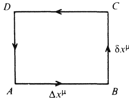
Fig. 3.13. A round trip by parallel transport.
