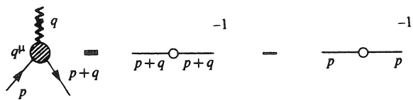
Fig. 7.4. Ward–Takahashi identity.
