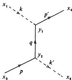
Fig. 6.9. \pi^+ p scattering.
