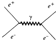
Fig. 7.7. Electron-positron scattering to order e^2 .
