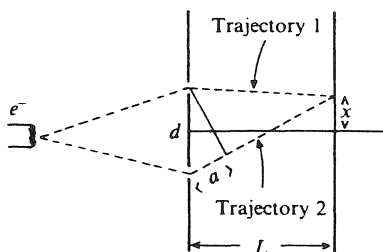
Fig. 3.6. The 2-slit interference experiment with electrons.
