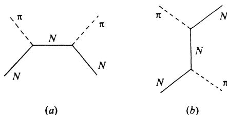
Fig. 6.8. Connected Feynman diagrams for pion–nucleon scattering, to second order.
