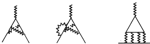
Fig. 9.12. Examples of irreducible vertex diagrams.
