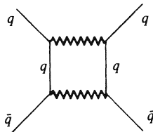
Fig. 7.9. Quark–antiquark scattering to order g^4 in QCD.
