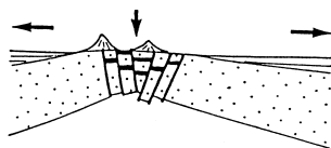
MAJOR RIFTING (REGIONAL TENSION)
