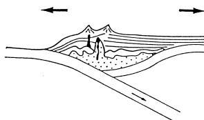
SUBDUCTION (REGIONAL TENSION)
