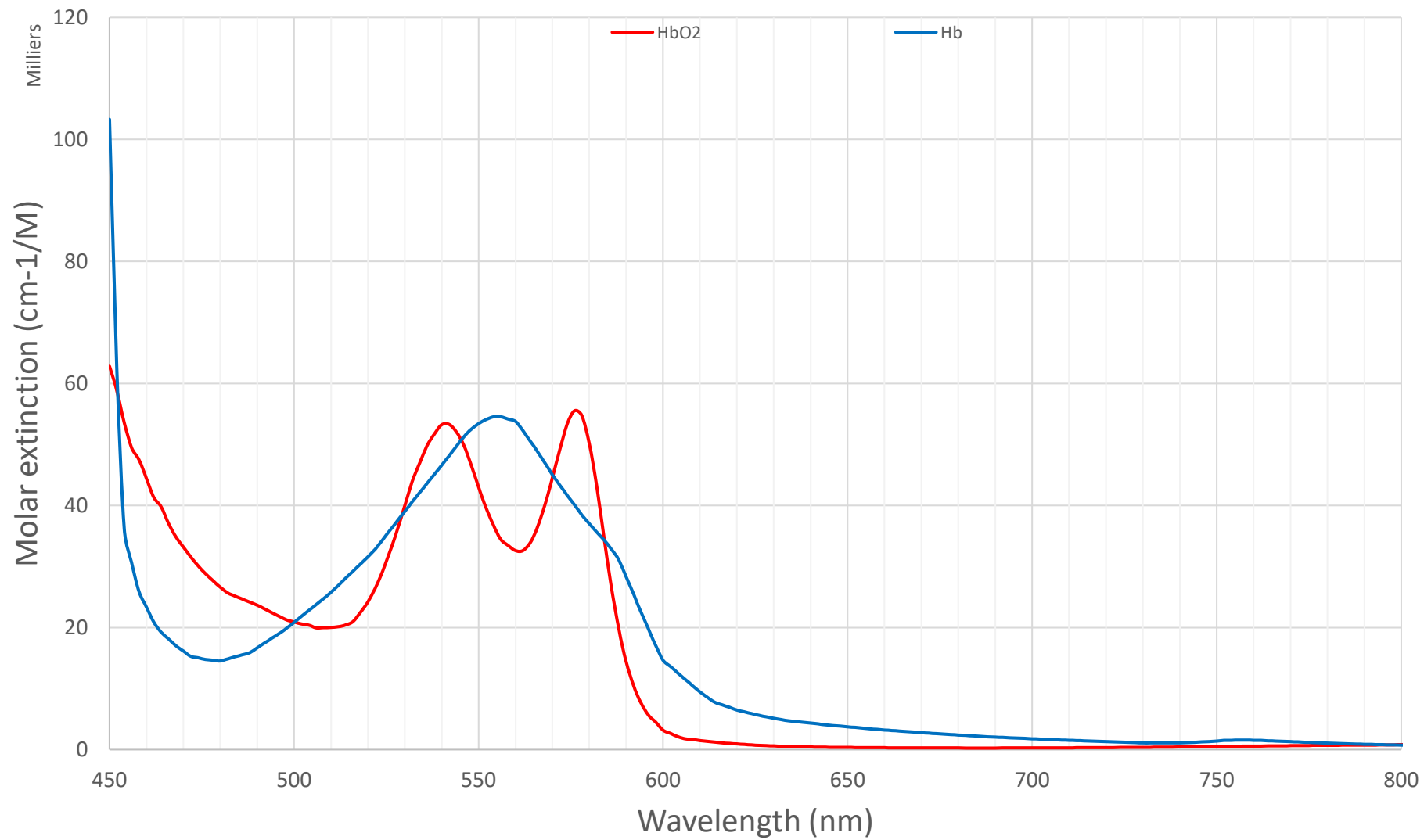
Extinction coefficient of Hb and HbO 2
