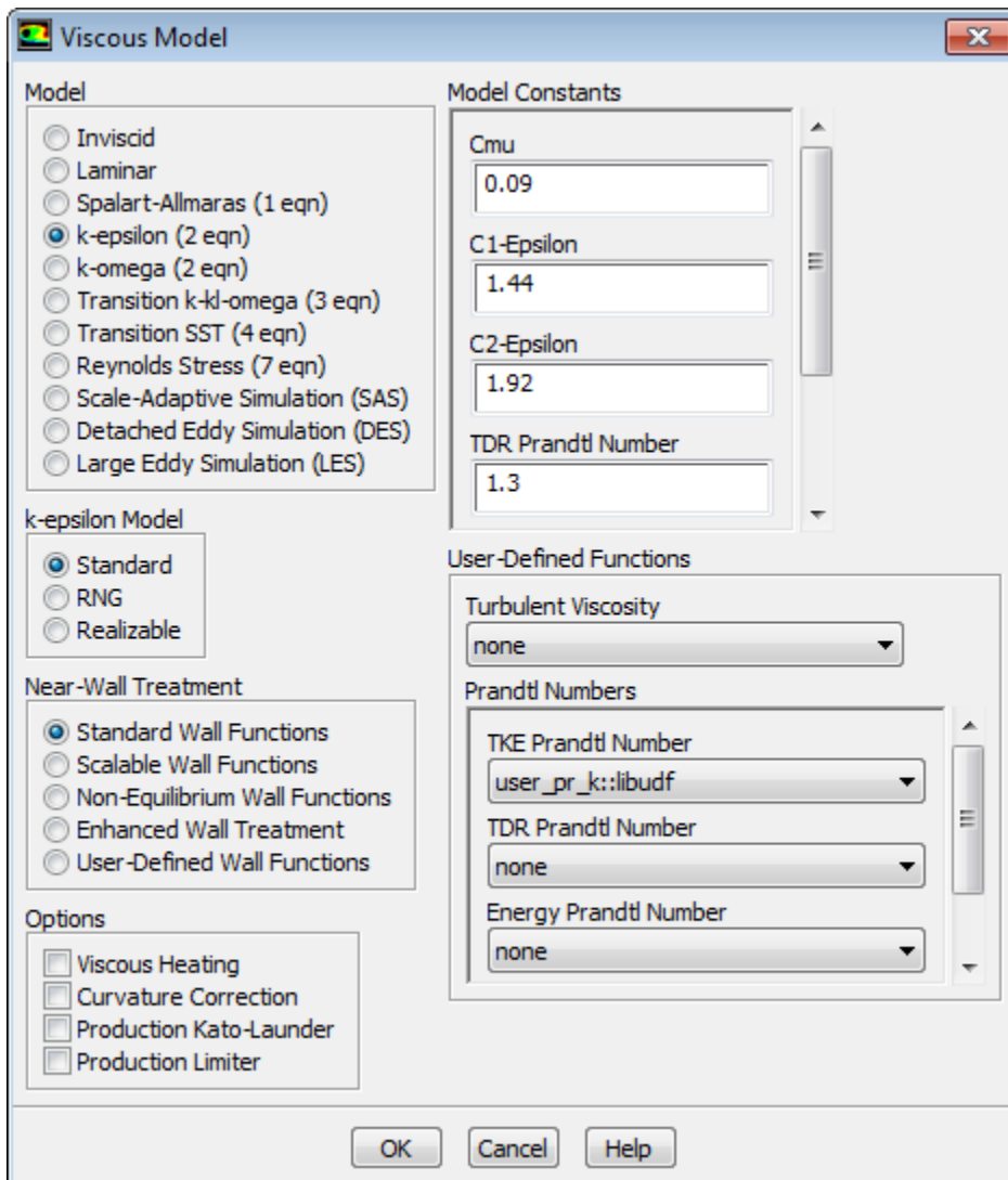
Figure 6.36: The Viscous Model Dialog Box
