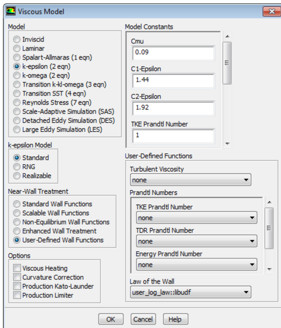
Figure 6.66: The Viscous Model Dialog Box
