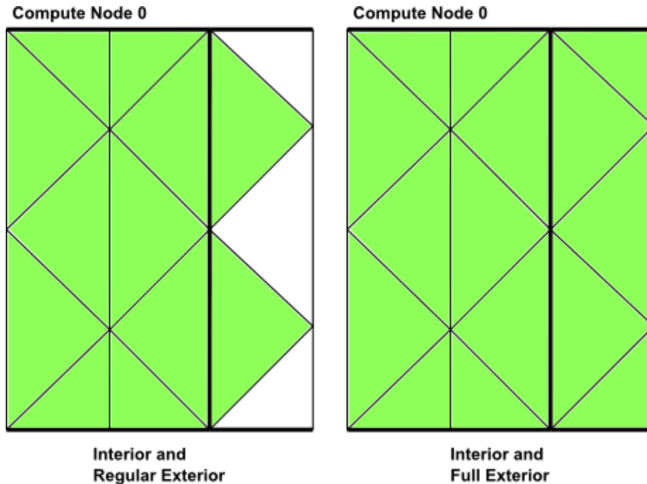
Figure 7.13: Looping Over Both Interior and Exterior Cells in a Partitioned Mesh Using begin_c_loop_int_ext
