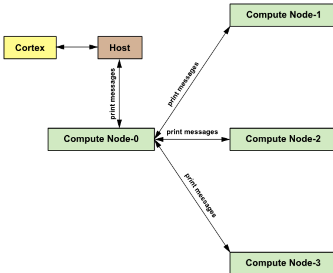
Figure 7.5: Example of Command Transfer in Parallel ANSYS Fluent
