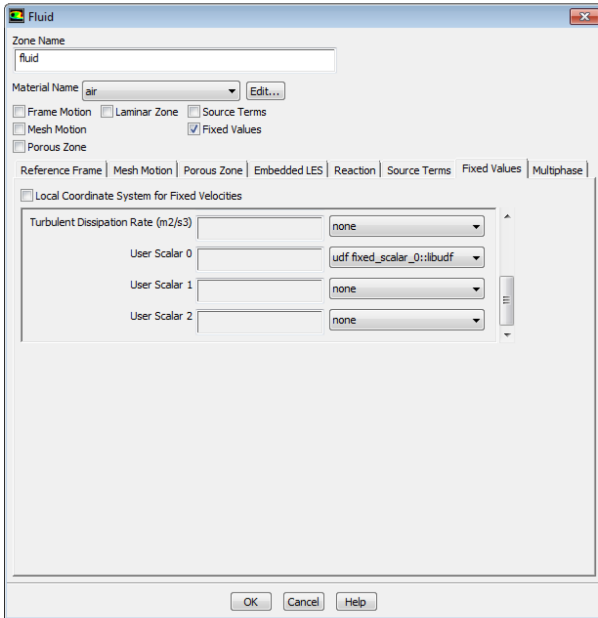
Figure 6.38: The Fluid Dialog Box with Fixed Value Inputs for User-Defined Scalars
