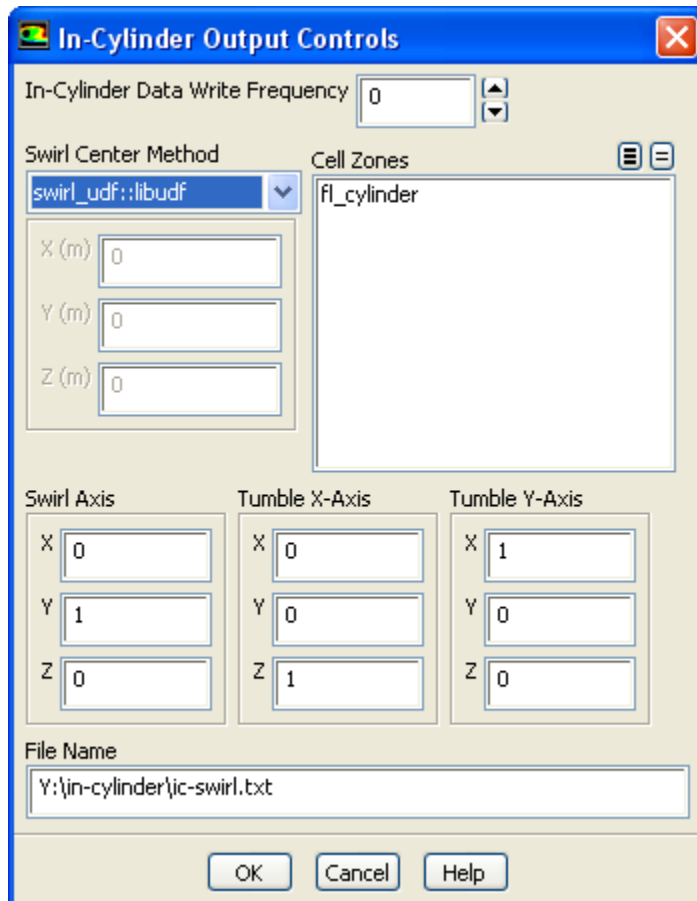
Figure 6.100: In-Cylinder Output Controls Dialog Box
