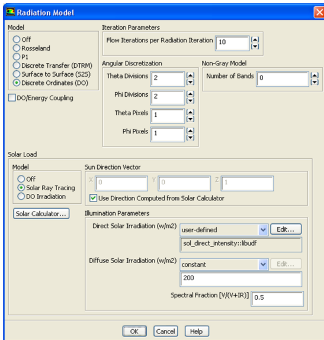
Figure 6.45: The Radiation Model Dialog Box
