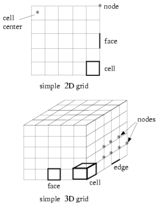
Figure 1.1: Mesh Components
