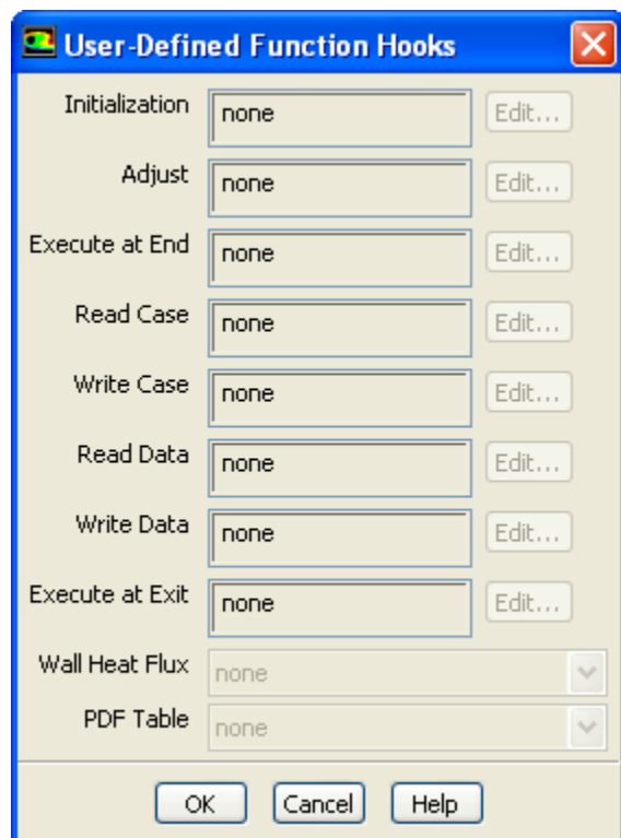
Figure 6.34: The User-Defined Function Hooks Dialog Box
