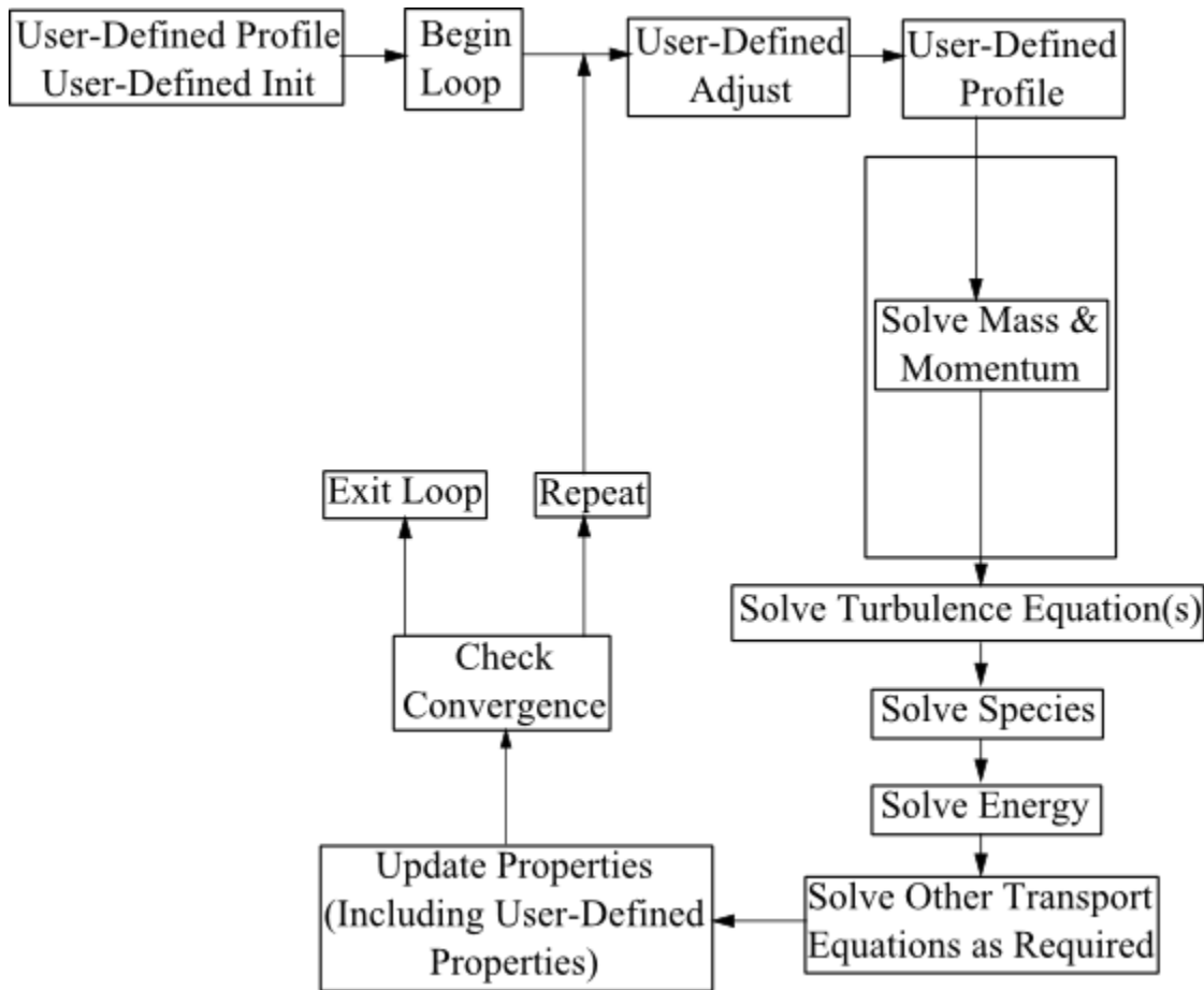
Figure 1.3: Solution Procedure for the Pressure-Based Coupled Solver
