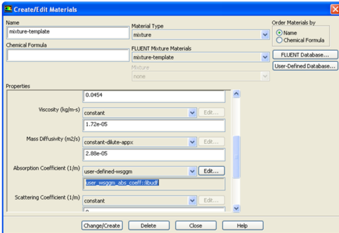
Figure 6.67: The Create/Edit Materials Dialog Box
