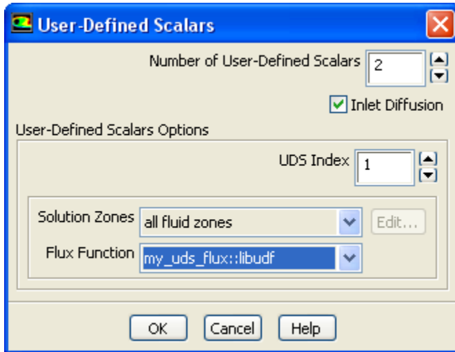
Figure 6.108: The User-Defined Scalars Dialog Box
