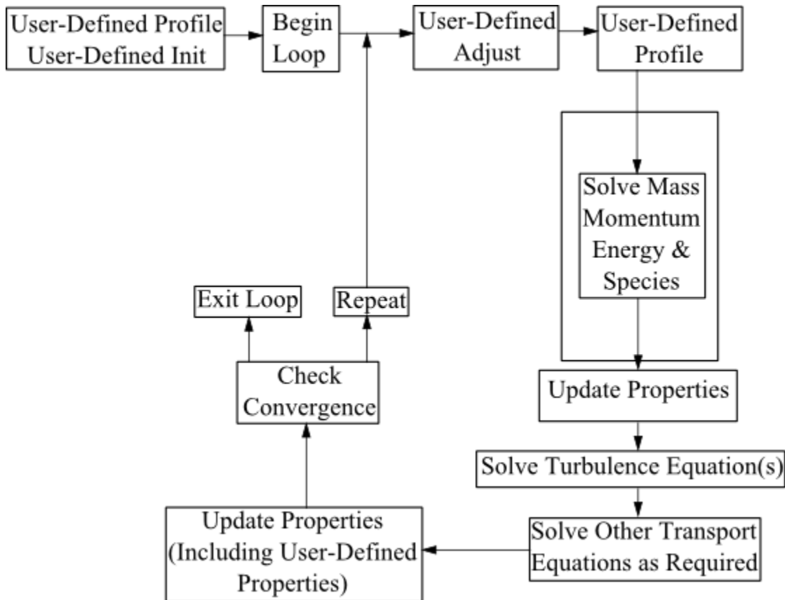
Figure 1.4: Solution Procedure for the Density-Based Solver
