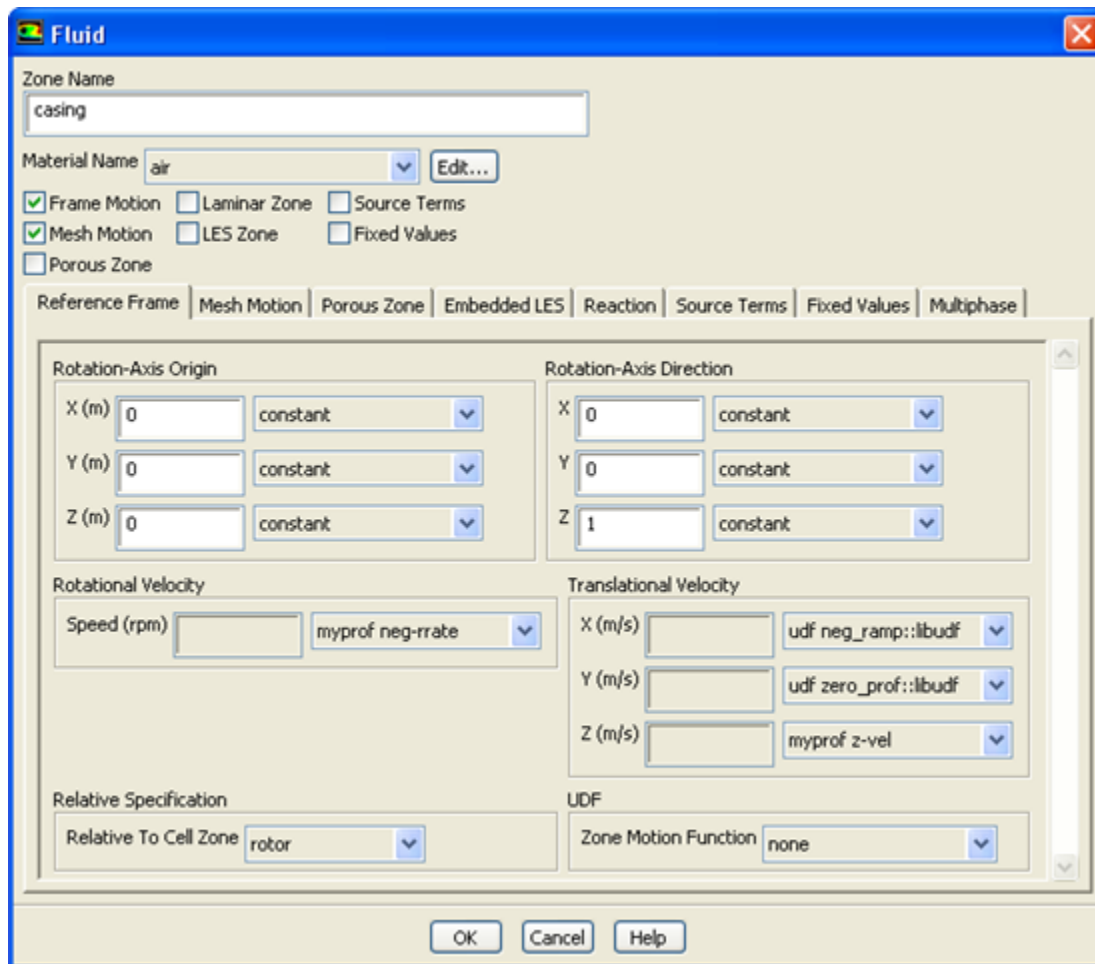
Figure 6.61: The Fluid Dialog Box
