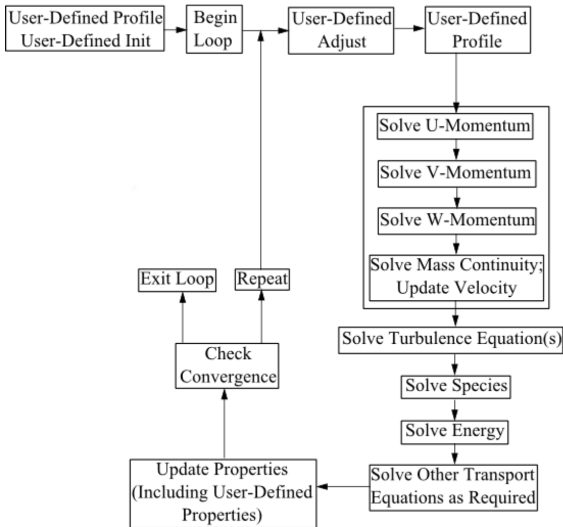
Figure 1.2: Solution Procedure for the Pressure-Based Segregated Solver
