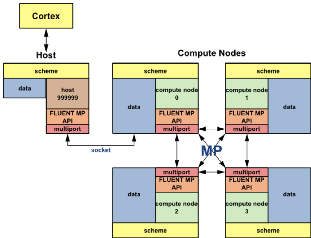
Figure 7.4: Parallel ANSYS Fluent Architecture
