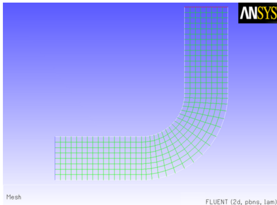
Figure 8.10: The Mesh for the Elbow Duct Example
