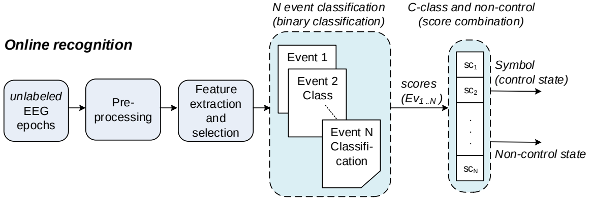
Fig. 8. Online classification architecture of a self-paced P300-based BCI system. EEG signal is segmented into epochs associated to each event, and preprocessed (filtering and normalization). Feature extraction and selection is applied and then a binary classifier is applied to each event. Then, the output scores are combined, identifying the symbol mentally selected by the user or a non-control state.
