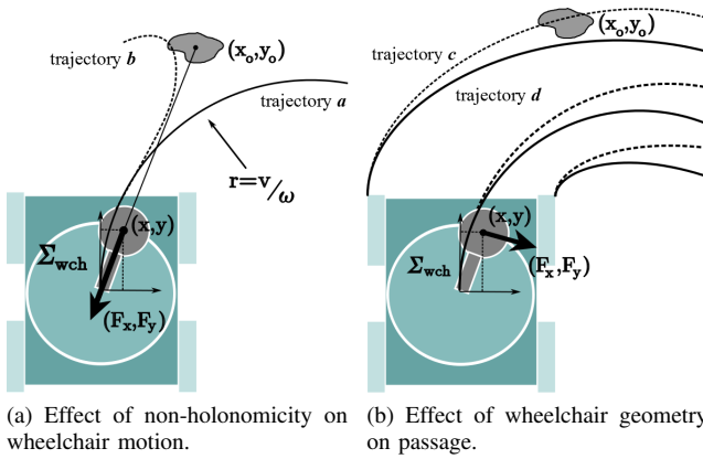
Fig. 4: Need to incorporate accurate kinematic wheelchair model into haptic guidance algorithms.
