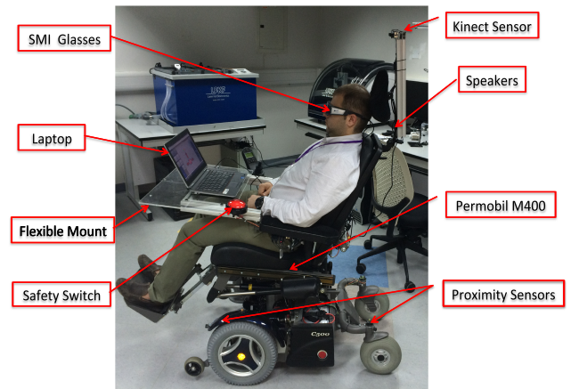
FIGURE 15. A snapshot of the complete system.
