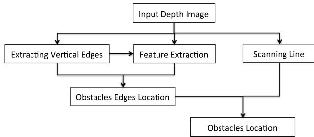
FIGURE 7. The diagram of the obstacle location procedure.
