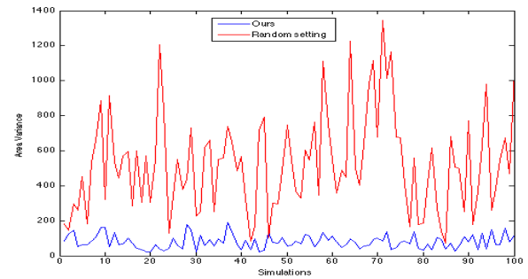
FIGURE 11. The variance of the areas of the two settings in each simulation run. The random setting shows great instability in comparison with our method.
