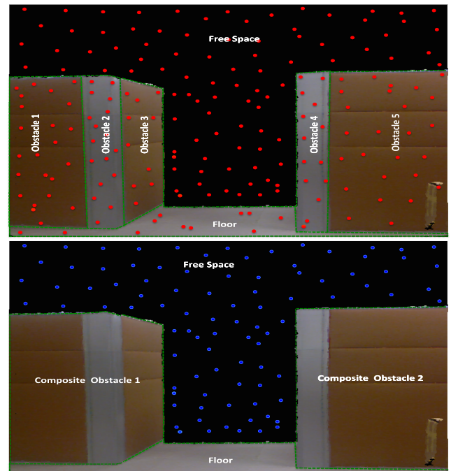
FIGURE 9. Local target generation phase (Top: Uniformly distributed points cover the entire surface, Bottom: The “Good Points” as the blue dots).
