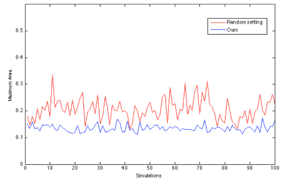
FIGURE 12. The maximum covered area as percentage (%) of the entire available space.
